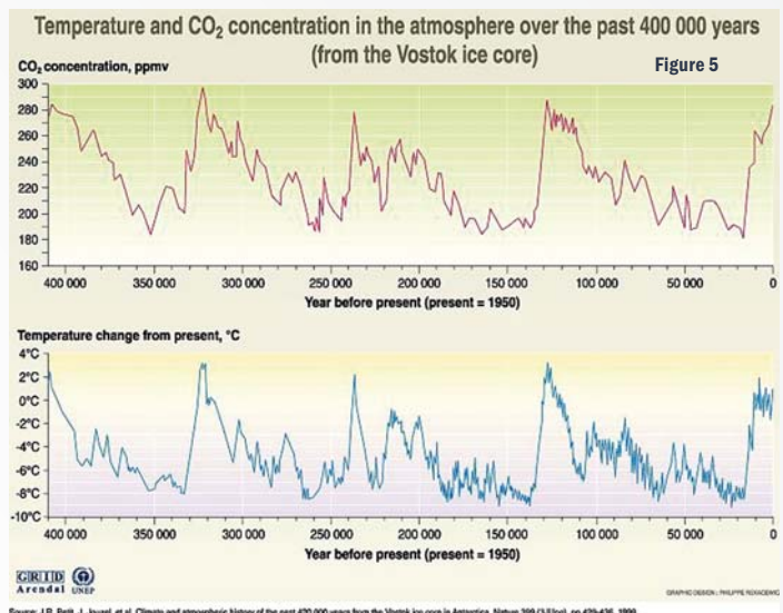
Source: J.R. Petit, J. Jouzel, et al. Climate and atmospheric history of the past 400 000 years from the Vostok ice core in Antarctica, Nature 399 (344), pp 429-436, 1999.
